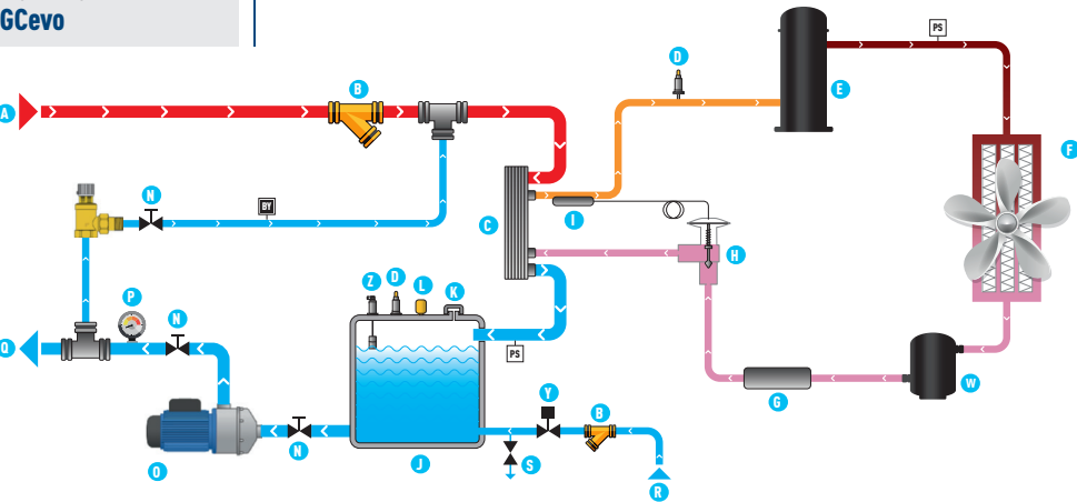
FLOW DIAGRAM GCevo
